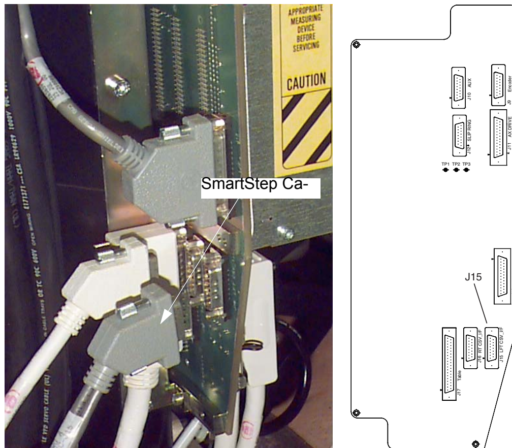
Figure 2-9 Locating connectors J15 (grey) on STC backplane
