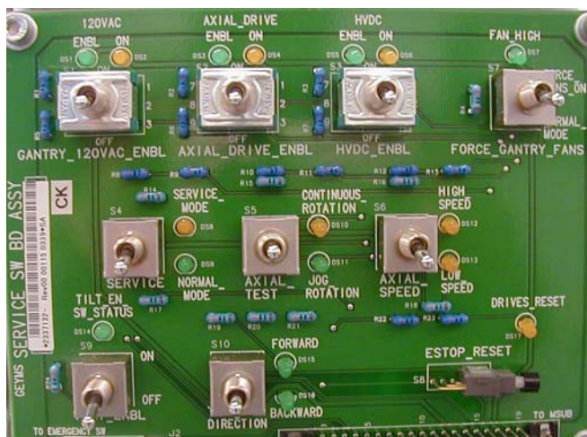
Figure 3-3 LightSpeed Gantry Service Switches
