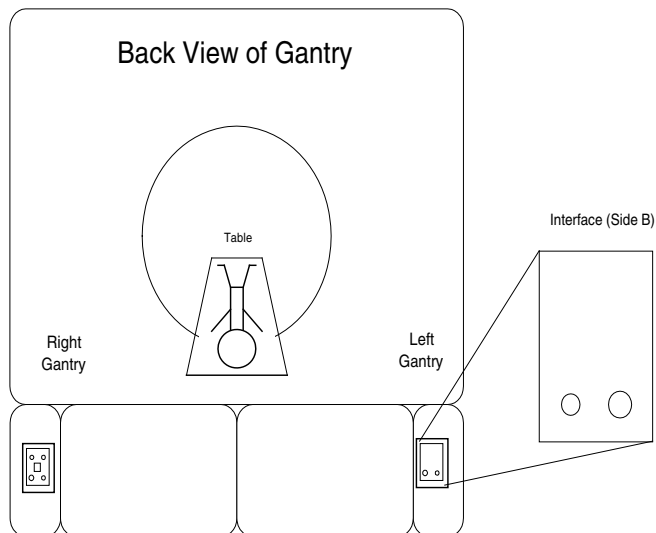
Figure 2-2 Gantry Connections
